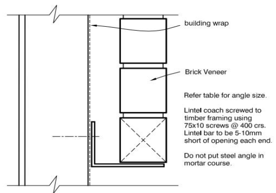
FIG.10 LINTEL BAR - FIXED TO FRAME
