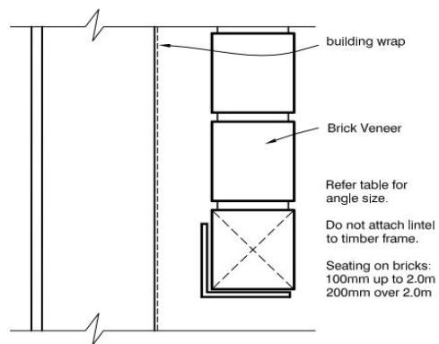
FIG.9 LINTEL BAR - TRADITIONAL
