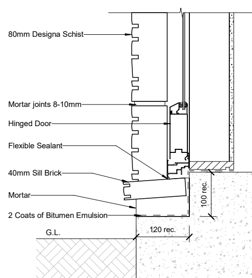
Fig. 5 Designa Schist - Brick Door Sill
