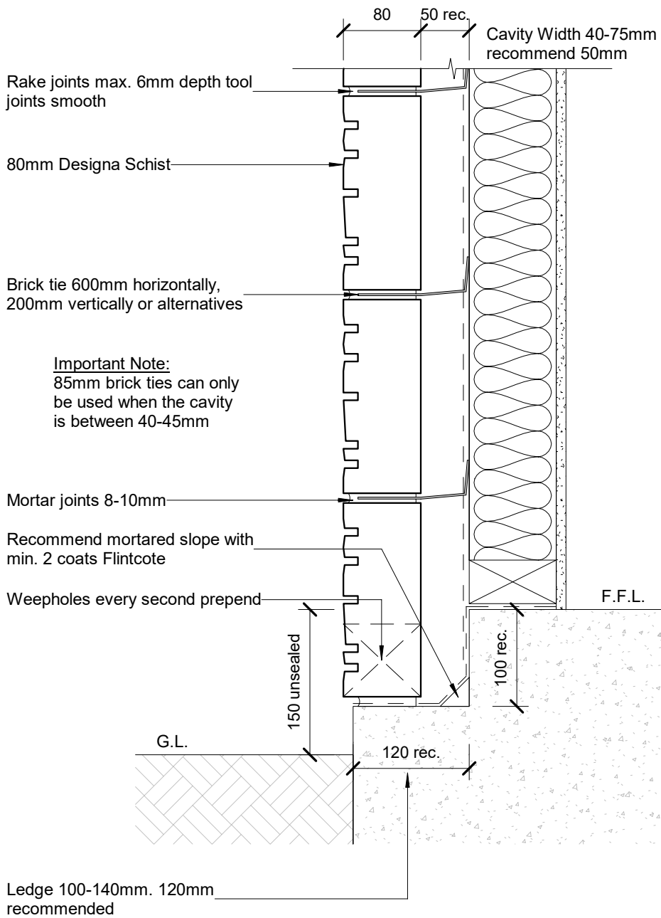
Fig. 1 Standard Designa Schist Veneer
