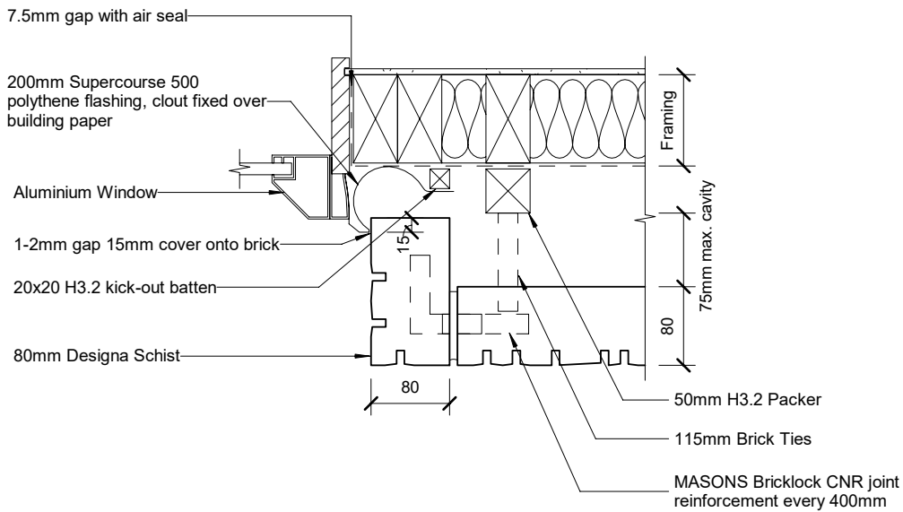
Fig. 11 Designa Schist - Deep Reveal Window Jamb - Double Stud Framing
