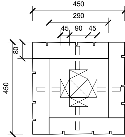
90 x 90mm H5 timber post with 90 x 45 H3.2 packers. Note: Use Quality timber and do not fill with concrete.
