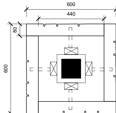
190 x 190mm reinforced block column with 90 x 45mm H3.2 packers. Use 135mm brick ties at each course.
