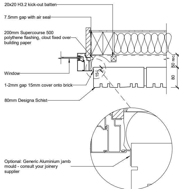
Fig. 9 Designa Schist - Window Jamb - Aluminium
