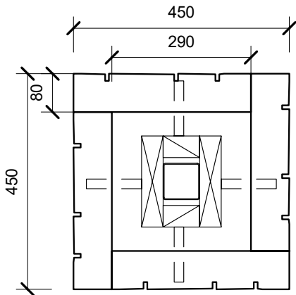
76 x 76 galv. steel box section, with 190 x 45mm H3.2 bolted to post. Use 115mm brick ties.
