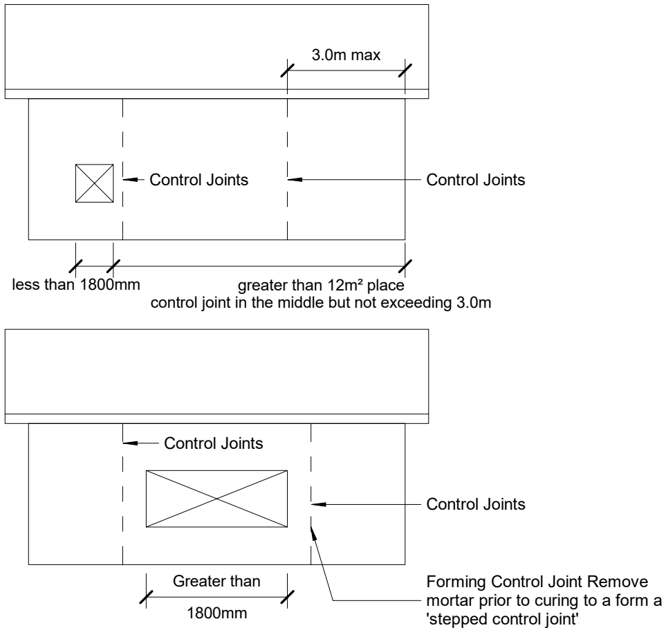
Fig. 12 Designa Schist - Control Joints
