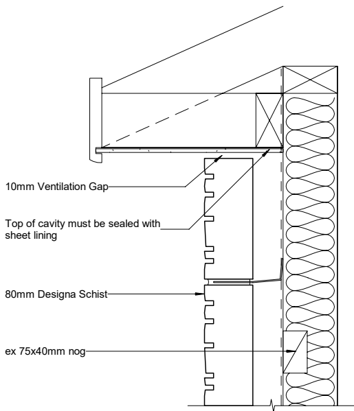
Fig. 4 Designa Schist - Flat Soffit & 150mm Frieze Board
